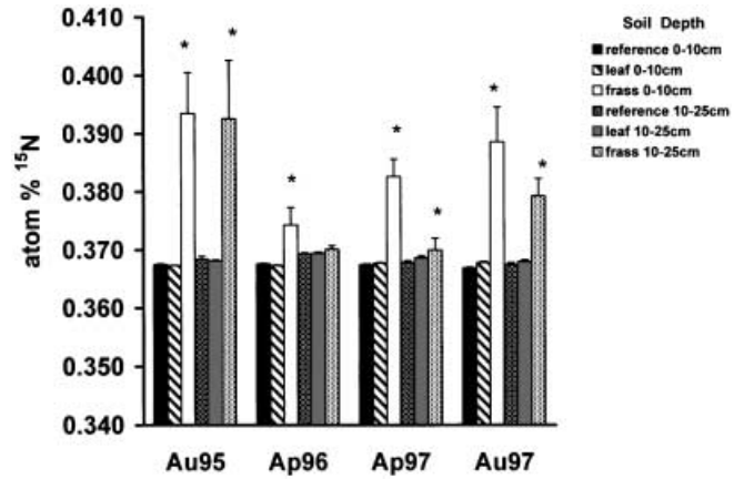
Fig. 1 Mean ( \pm SE) of atom % ^{15}\text{N} for surface (0–10 cm) and sub-surface (10–25 cm) soils. An asterisk indicates a significant ( P < 0.05 ) difference
