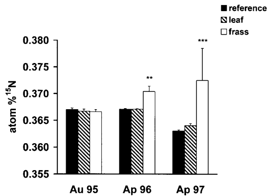
Fig. 2 Mean ( \pm SE) atom % ^{15}\text{N} of leaching losses for \text{NO}_3^- in ion exchange resin extracts. Asterisks ( *P < 0.05 , **P < 0.01 , ***P < 0.001 ) indicate significant differences between the treatments and reference within a sampling period
