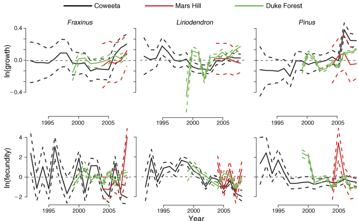
FIG. 10. Posterior medians and 95% CIs for year effects \mathbf{b}_j , (Eq. 8b) for three species in the three regions. Separate year effects were used for Blue Ridge (black), Mars Hill (red), and Piedmont (green). Note the scale difference: the range for fecundity is four times that for diameter growth.
