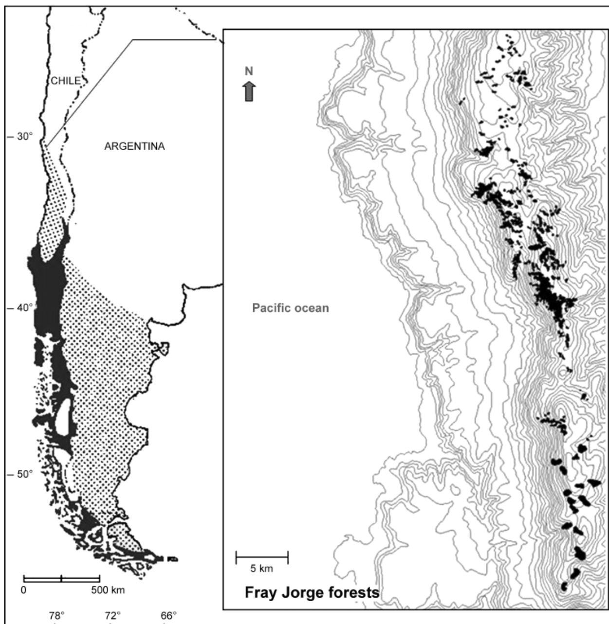
Fig. 1 Study site and overview of the Fray Jorge landscape showing the mosaic of forest patches (dark spots) on a coastal mountaintop of semiarid Chile (right side). Topographic lines of equal elevation (every 50 m) are shown. Forest patches are found above 500 m. The main distribution of southern temperate rain forests (dark shading) and semiarid ecosystems (stippled) in southern South America are shown on the left side.
