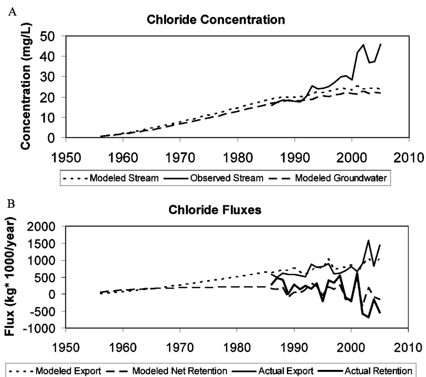
FIGURE 5. Model results: (A) chloride concentrations (mg/L) and (B) chloride fluxes (1000 kg/year).
